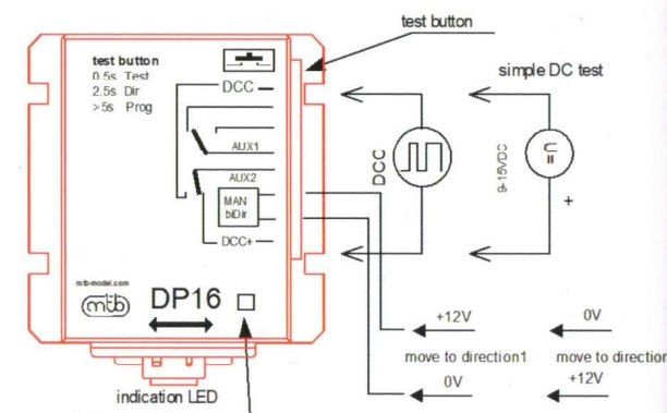
DCC schematic - DP16
