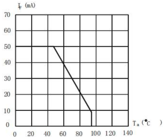
DC Forward Current VS Temperature
